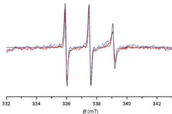
Figure 3. EPR spectra of the spin-labelled peptide (CGK(SL)GHHHHHHH (black), RBD-CGK(SL)GHHHHHHH (red), and RBD-CGK(SL)GHHHHHHH in complex with Ras(GppNHp) (blue). Experimental conditions: The spin-labelled peptide was measured in 6 M guanidinium hydrochloride buffered with 100 mM NaOAc at pH 4.0. RBD and RBD-Ras complex have been measured in 50 mM Tris HCl, 100 mM NaCl, 5 mM MgCl 2 at pH 7.4. Measurements were performed with a home-built EPR spectrometer equipped with a Bruker dielectric cavity with the following settings: microwave power 0.4 mW, modulation amplitude 0.1 mT, scan time 60 s, 10 scans accumulated for RBD and RBD in complex with Ras.
