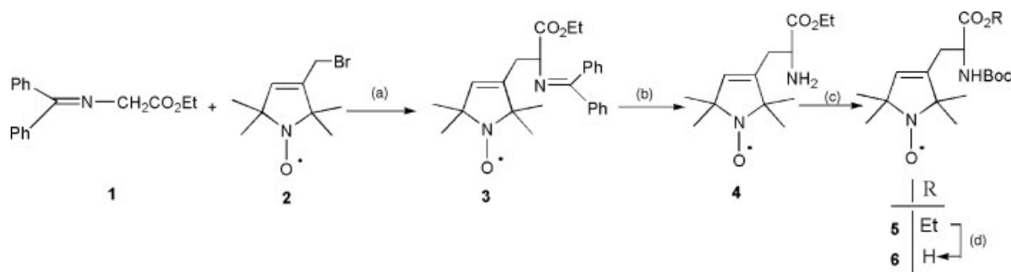
Scheme 2. The reaction scheme for the synthesis of the paramagnetic Boc-protected amino acids 5 and 6 . (a) 10% aq. NaOH, CH 2 Cl 2 , Bu 4 NHSO 4 ; (b) 5% aq. H 2 SO 4 , EtOH; (c) Boc 2 O, THF; (d) 10% aq. NaOH, EtOH.
