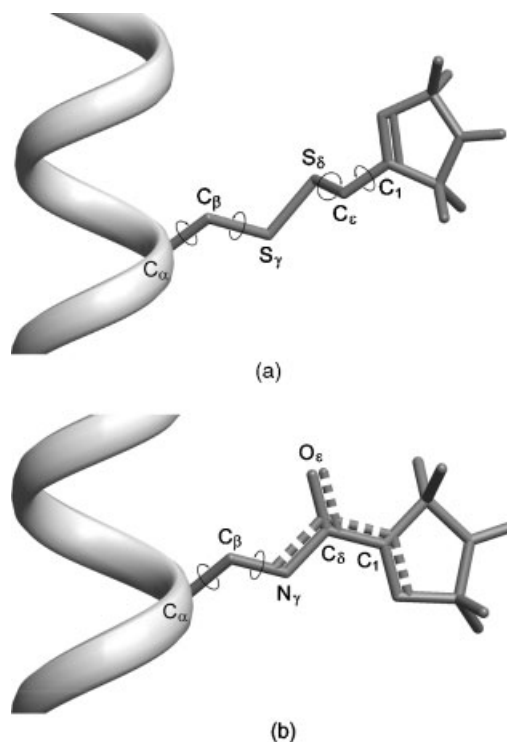
Figure 1. Conformational space of two spin-labelled amino acids (MTSSL (a) and II (b)). The double bond character of the peptide bond in conjugation with the double bond in the five-membered ring is indicated by dots.
