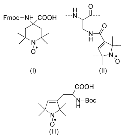
Scheme 1. Chemical structures of nitroxide-containing amino acids.
