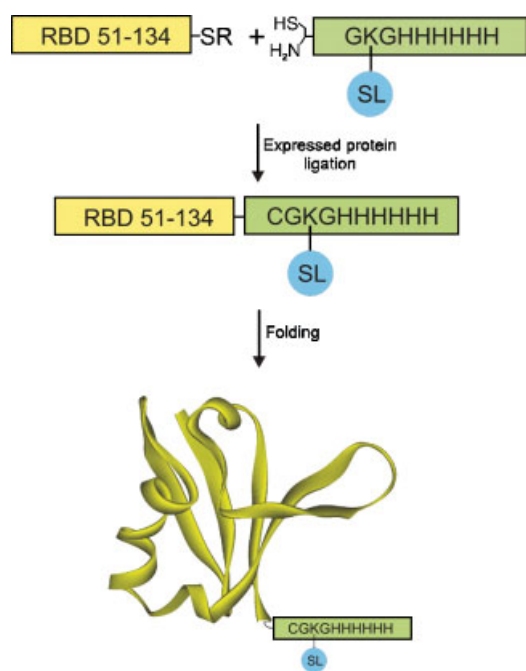
Figure 2. Strategy for the C-terminal spin labelling of RBD.
