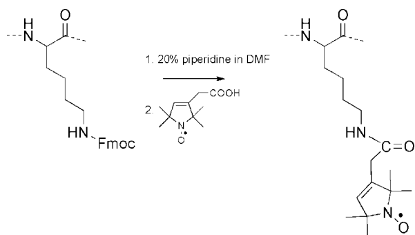
Scheme 3. Coupling of spin label to the \epsilon -amino group of lysine. 19
