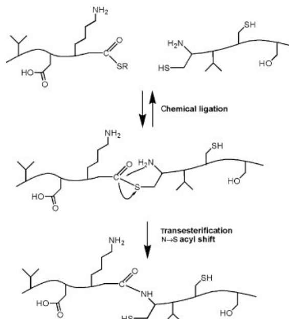
Scheme 4. Mechanism of native and expressed protein ligation.
