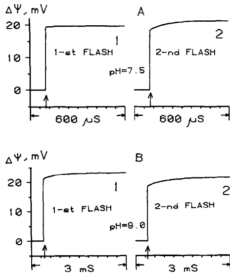
Fig.1. Generation of electric potential by Rhodobacter sphaeroides chromatophores on the first (1) and second (2) laser flashes at pH 7.5 (A) and pH 9.0 (B). The incubation medium contained 1 mM ferrocyanide, 50 \mu M N,N,N',N' -tetramethyl- p -phenylenediamine, 5 \mu M antimycin A, 3 \mu M myxothiazol and 20 mM buffer (HEPES at pH 7.5 and bis-tris -propane at pH 9.0). The arrows indicate laser flashes. The second flash was given 2 s after the first.
