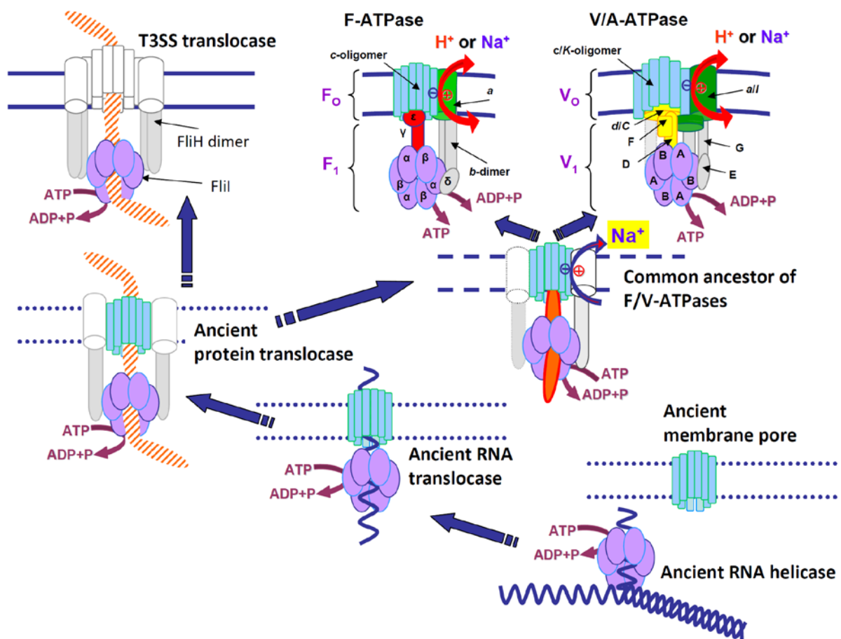
Figure 2. The proposed scenario of evolution from separate RNA helicases and primitive membrane pores, via membrane RNA and protein translocases, to the ion-translocating membrane ATPases. The color code is as in Figure 1; ancient/uncharacterized protein subunits are not colored. The striped shapes denote the translocated, partially unfolded proteins. The presence of two peripheral stalks in the primordial protein translocase and the flagellar/T3SS systems is purely hypothetical and based on the consideration that a system with one peripheral stalk would be unstable in the absence of the translocated substrate. The involvement of two FliH subunits in each peripheral stalk is based on the ability of FliH dimers to form a complex with one FliI subunit (Minamino and Namba 2004; Imada et al. 2007).
