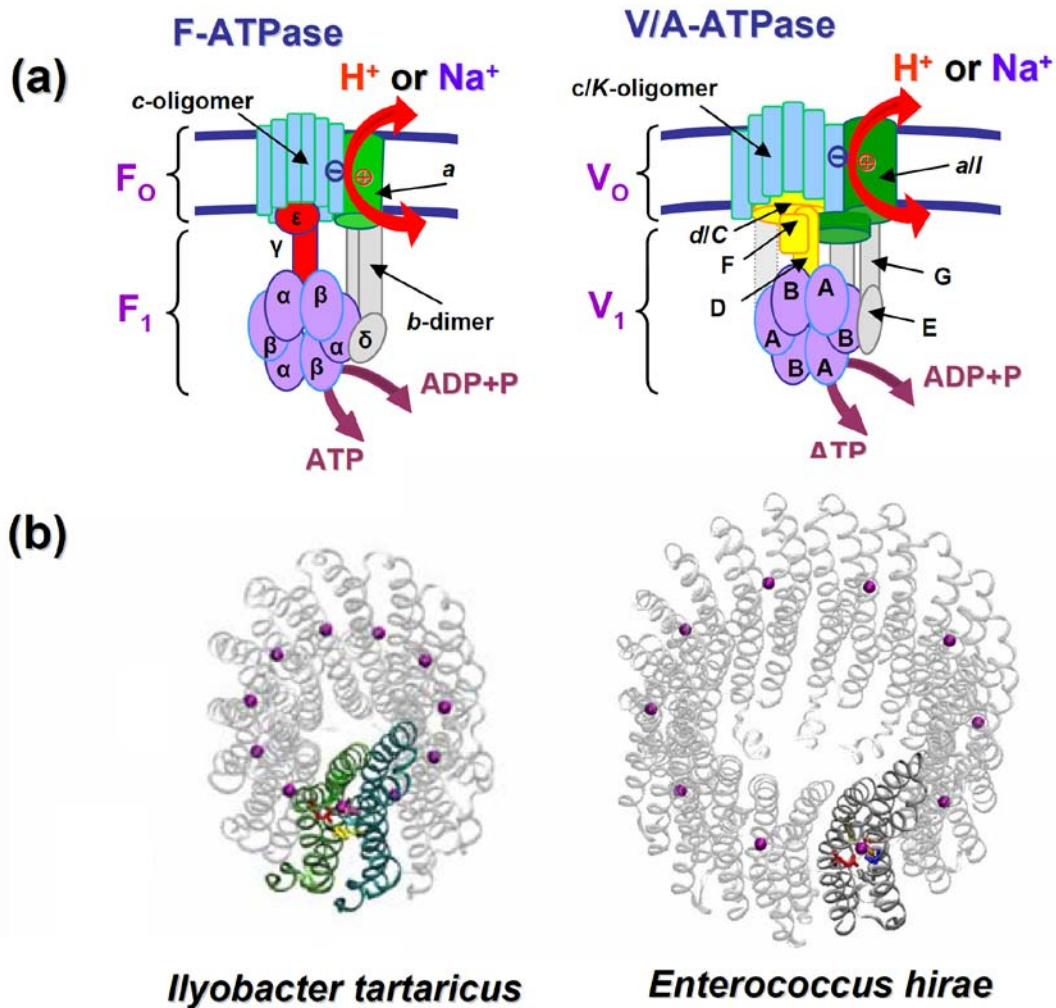
Fig. 1. Structure and evolutionary relationships of F-type and A/V-type ATPases. (a): modern F- and V-type ATPases; the minimal, prokaryotic sets of subunits are depicted; orthologous subunits are shown by the same colors and shapes, and non-homologous but functionally analogous subunits of the central stalk are shown by different colors. The a subunits that show structural similarity but might not be homologous (Mulikidjanian et al. 2007) are shown by distinct but similar colours; in the case of those V-ATPase subunits that are differently denoted in prokaryotes and eukaryotes, double notation is used: eukaryotic/prokaryotic. The composition of peripheral stalk(s) and their number in V-ATPases remains ambiguous, with values of up to 3 being reported (Esteban et al. 2008; Kitagawa et al. 2008). For further details, see refs. (Mulikidjanian et al. 2007; Mulikidjanian et al. 2009). (b) membrane rotor subunits of the Na + -translocating ATP synthases; left, undecamer of c subunits of the Na + -translocating F-type ATP synthase of Ilyobacter tartaricus (PDB entry 1YCE (Meier et al. 2005)); right, decamer of K subunits of the Na + -translocating V-type ATP synthase of Enterococcus hirae (PDB entry 2BL2 (Murata et al. 2005)); both rings are tilted to expose the internal pore; in I. tartaricus , Na + ions (purple) crosslink the neighbouring subunits, whereas in E. hirae the Na + ions are bound by four-helical bundles that evolved via a subunit duplication (see also (Mulikidjanian et al. 2008b; Mulikidjanian et al. 2009)).
